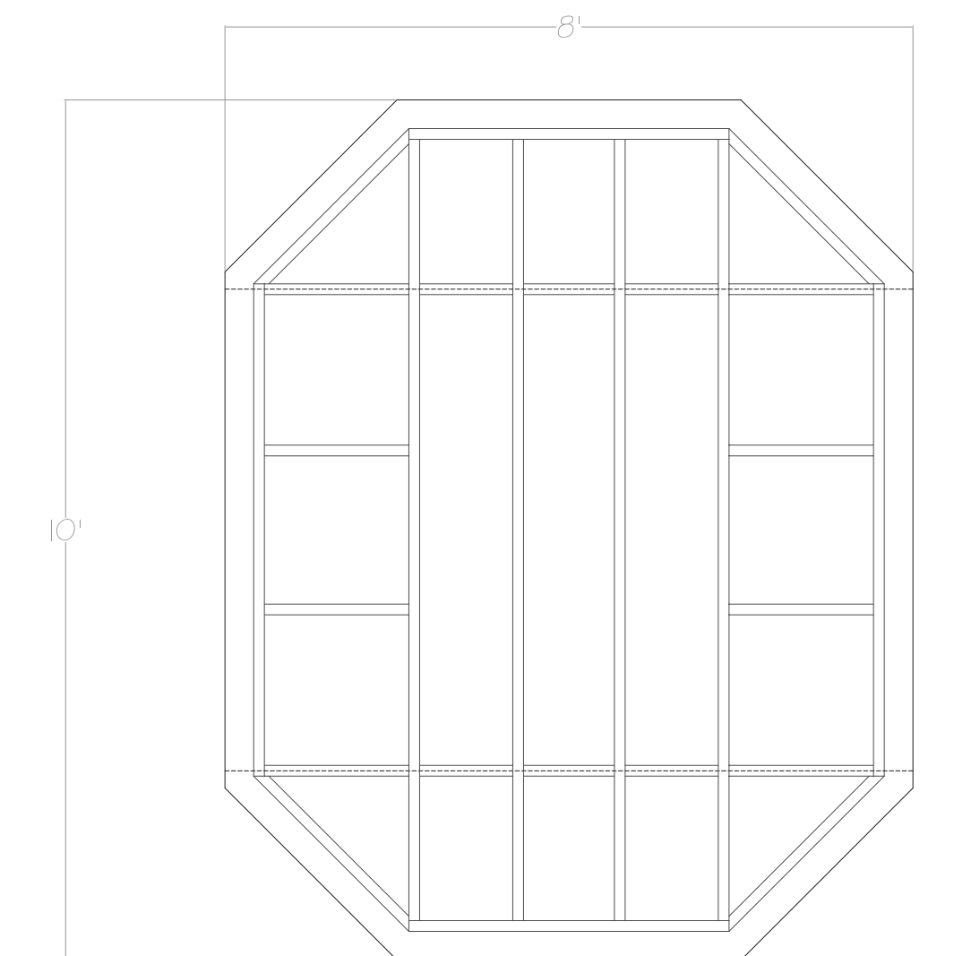
8 12 TOP PLATFORM FRAMING (OFFSET IS 4") ***SCALE: 1/2" = 1'-0"***
