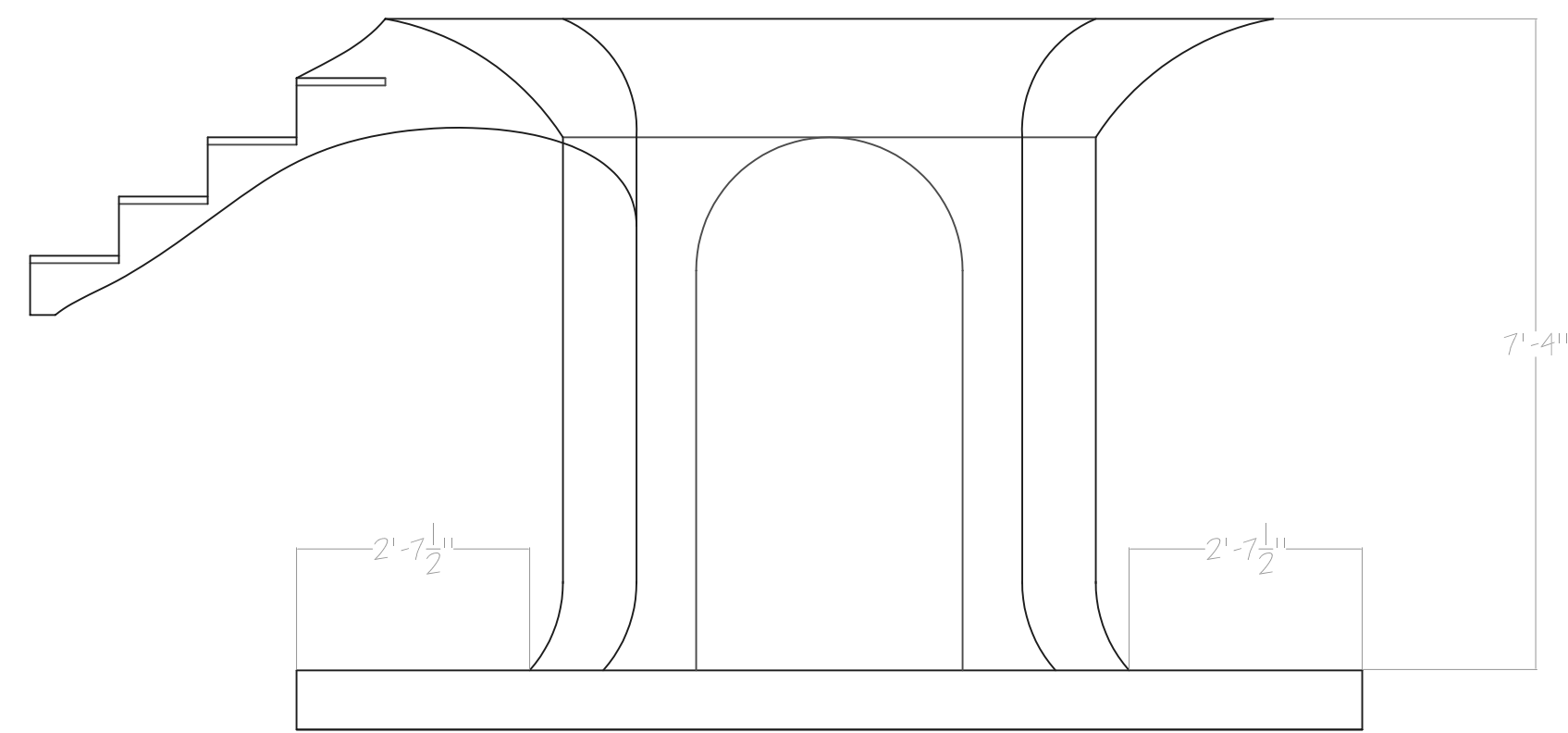
1 12 SOME BIG THING SIDE 'A' ***SCALE: 1/2" = 1'-0"***
