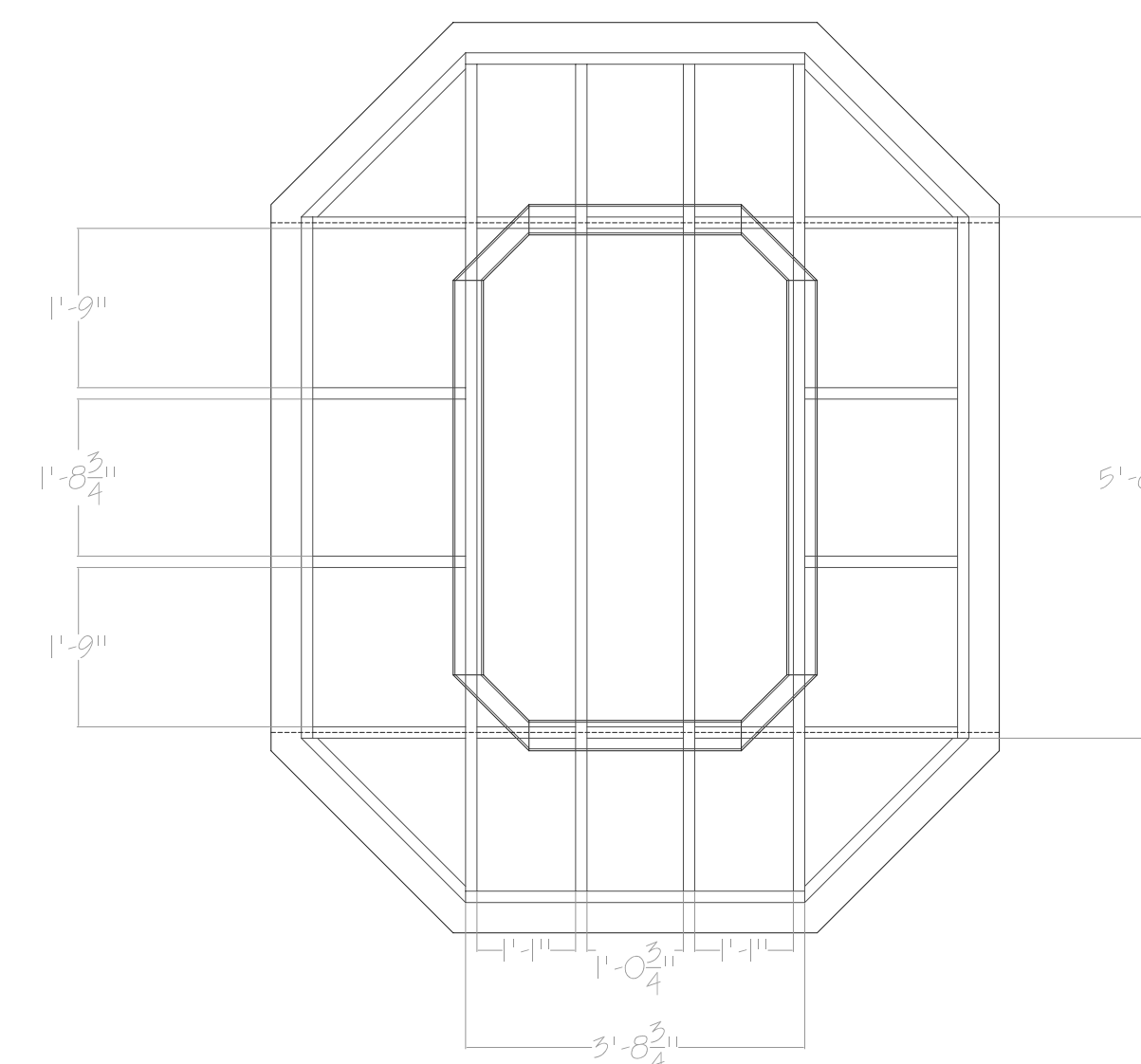
7 12 TOP VIEW COMPOSITE ***SCALE: 1/2" = 1'-0"***
